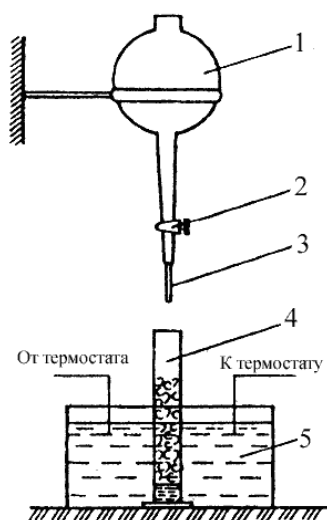
Figure 3 – Ross-Miles device
